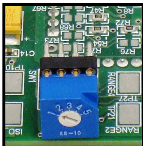
Figure 3-6. PPM Range Select Switch
